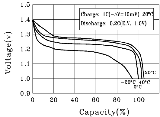
DISCHARGE CHARACTERISTICS AT DIFFERENT TEMPERATURE
