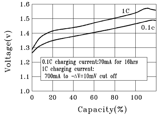
CHARGE CHARACTERISTICS
