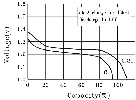
DISCHARGE CHARACTERISTICS
