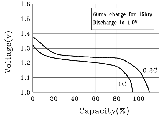
DISCHARGE CHARACTERISTICS
