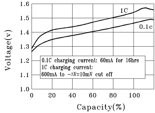
CHARGE CHARACTERISTICS
