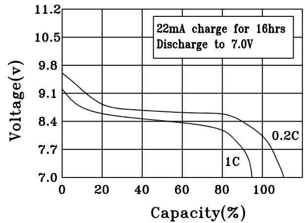
DISCHARGE CHARACTERISTICS
