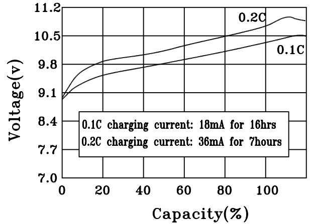
CHARGE CHARACTERISTICS
